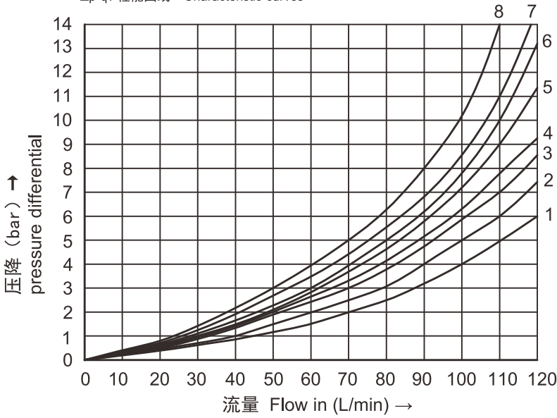
Δp-qv 性能曲线 Characteristic curves
