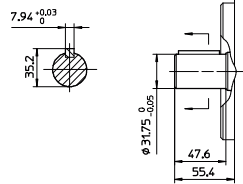
CODE XA - INTERMEDIATE FLANGE SAE "A" FOR PFE-31
