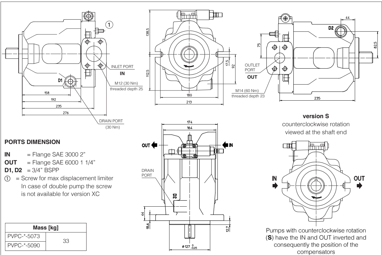
SHAFT TYPE "1"
